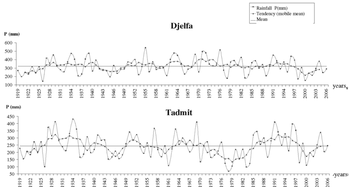
Fig. 1. Annual rainfall with tendencies (Benseghir, 2008).
