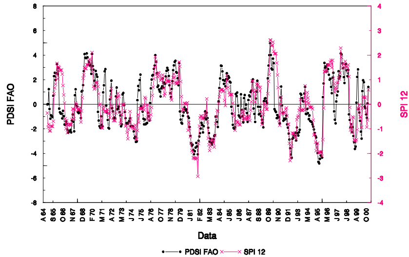
Fig. 4. Comparing the PDSI computed with the ETP-FAO56 and TAW=150 mm with the SPI computed for the time-scale 12-month at Beja, for the period 1965-2000.
