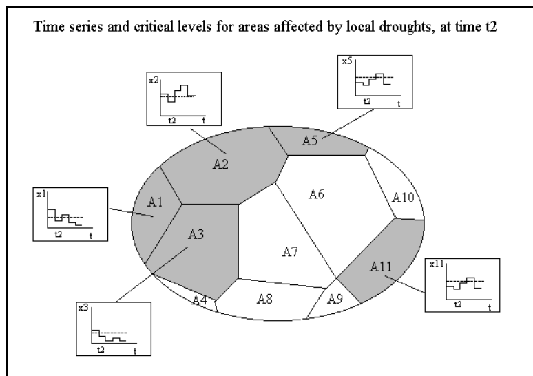
Fig. 5. Regional drought identification
