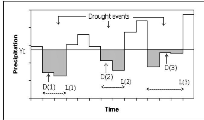
Fig. 3. Characteristics of local drought events with the theory of runs
