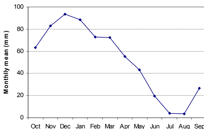
Fig. 2. Monthly mean areal precipitation in Alentejo from 49 rainfall stations for 1931/32 to 1998/99
