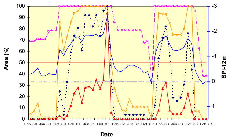
Fig. 6. Time evolution of the areal coverage relative to mild (—□—), moderate (—×—), severe (···◆···); and extreme (—▲—) drought categories and the SPI_{reg} (—) for the period Feb80–Feb84
