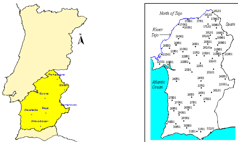
Fig. 1. Location of the Alentejo region and identification of rainfall stations utilized in the study
