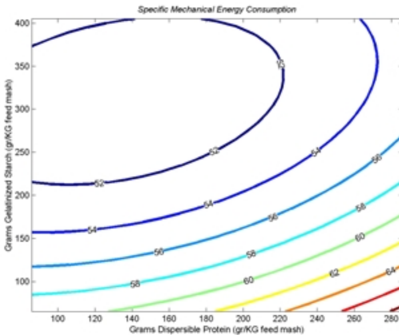
Fig. 4. Specific mechanical energy consumption (SME) (kJ/kg) of the pelletizer as a function of degree of gelatinization and dispersible protein.
