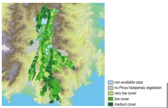
Fig. 5. Soil erosion risk map.
